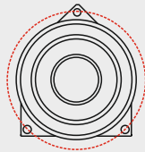
Bolt circle: 114mm
